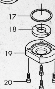
Pts. 17-20: Cover plate for Valve \geq DN 350
