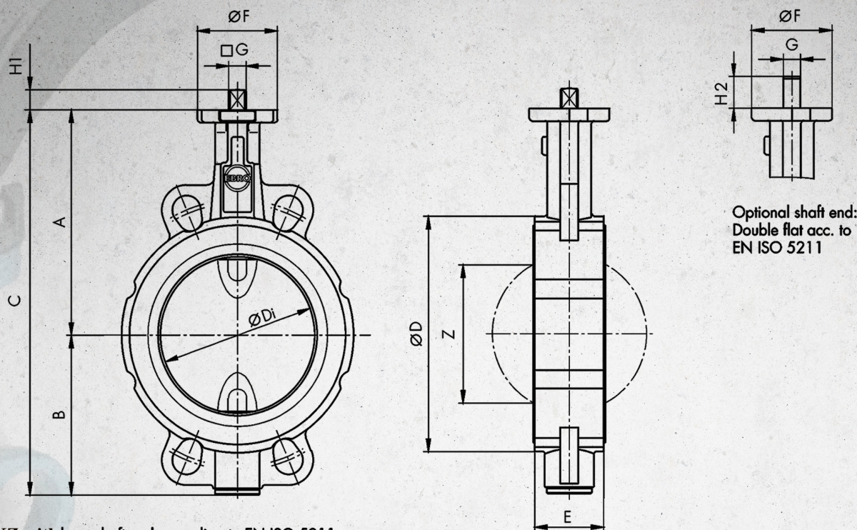
MKZ with bare shaft end according to EN ISO 5211
